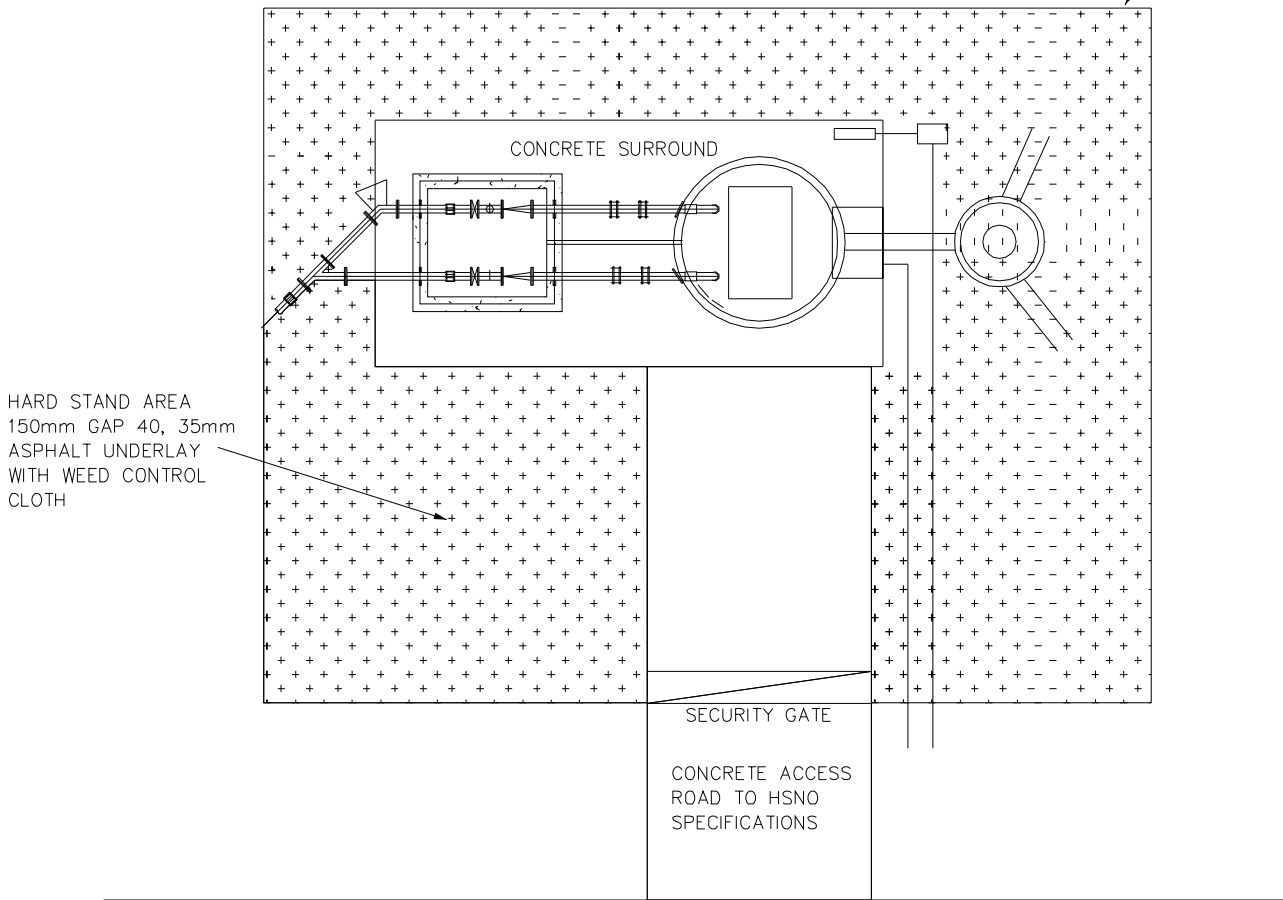
SITE LAYOUT
