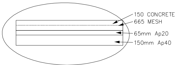
DRIVEWAY DETAIL
