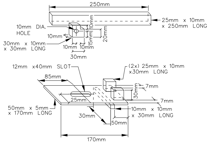
LATCH DETAIL
