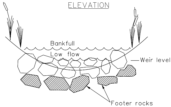
CROSS SECTION
