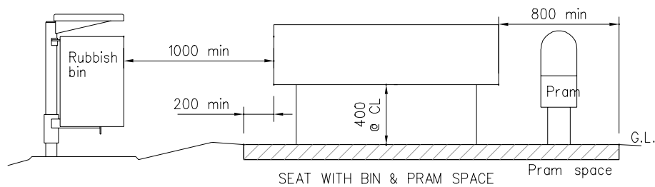
SEAT WITH BIN & PRAM SPACE
