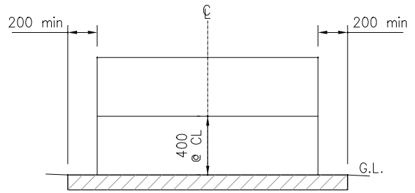
SEAT WITH BACK-FRONT ELEVATION
