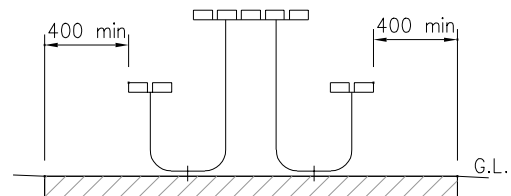
PICNIC TABLE-END ELEVATION
