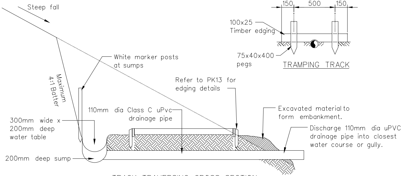
TRACK TRAVERSING CROSS SECTION
